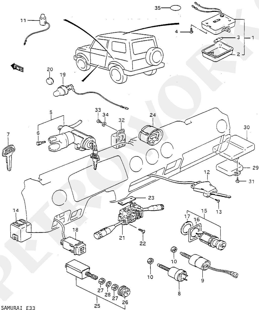
Dash Board Electrical Figure 43
